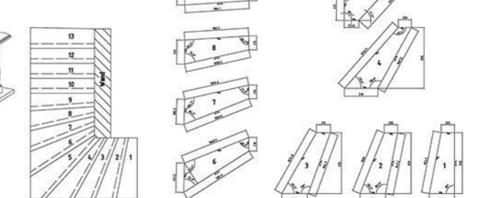
STAIR TREADS TO BE ASSEMBLED WITH BALUSTRADE
