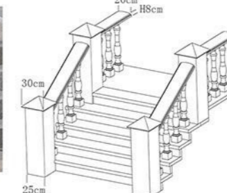
BALUSTRADE SKETCH
